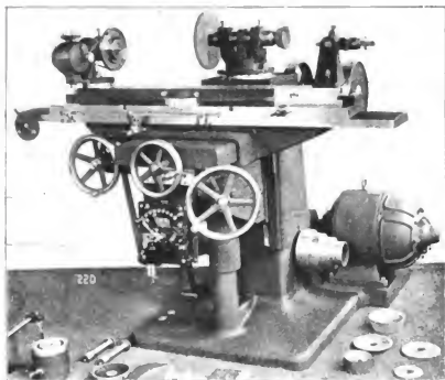
Fig. 3911. Tool Room Grinding Machine. Cincinnati Milling Machine Co.
